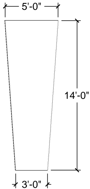
2 FRONT VIEW Scale: 3/16" = 1'-0"
