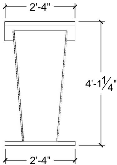
2 FRONT VIEW Scale: 1/2" = 1'-0"
